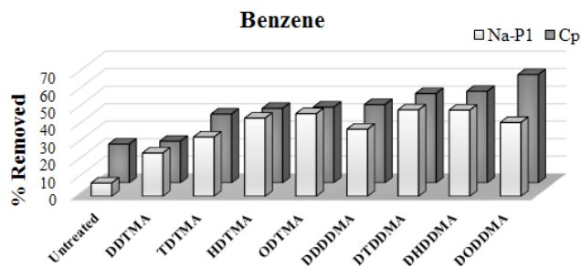
Fig. 6. Efficiency of benzene removal from aqueous solutions ( C_0 = 50 ppm, t = 2 h).
