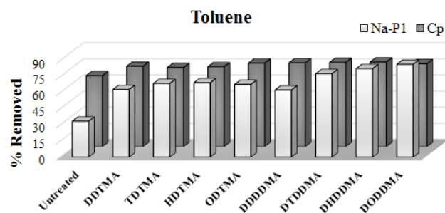
Fig. 7. Efficiency of toluene removal from aqueous solutions ( C_0 = 50 ppm, t = 2 h).
