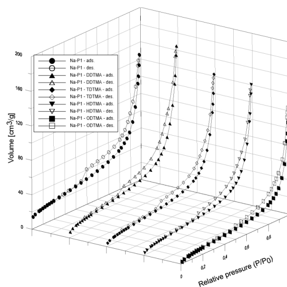
Fig. 3. Comparison of N 2 adsorption and desorption isotherms at -196°C for Na-P1 and its single modifications.
