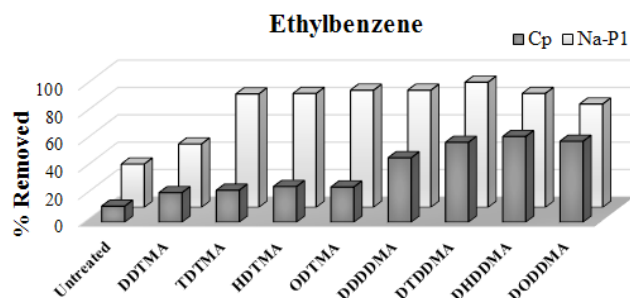
Fig. 8. Efficiency of ethylbenzene removal from aqueous solutions ( C_0 = 50 ppm, t = 2 h).
