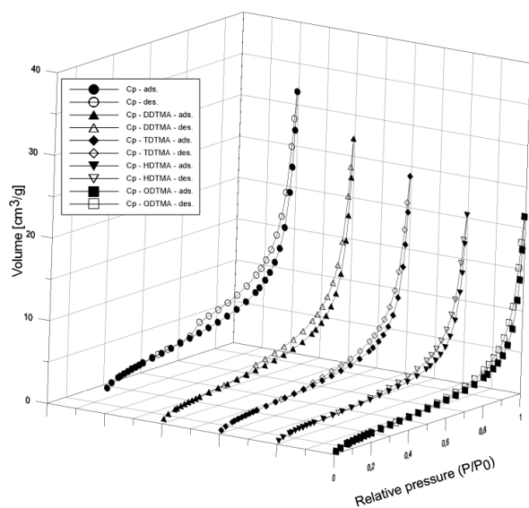
Fig. 4. Comparison of N 2 adsorption and desorption isotherms at -196°C for clinoptilolite and its single modifications.
