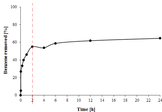
Fig. 5. Influence of reaction time on sorption efficiency. For example, Na-P1 modified with HDTMA in an amount of 1.0 ECEC, with a starting benzene concentration of 50 ppm.
