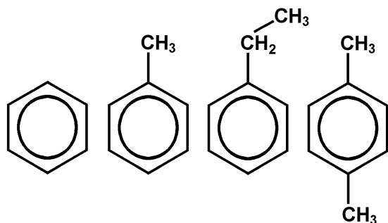
Fig. 1. Structural formulas of selected VOCs. From the left: Benzene, toluene, ethylbenzene and p-xylene.
