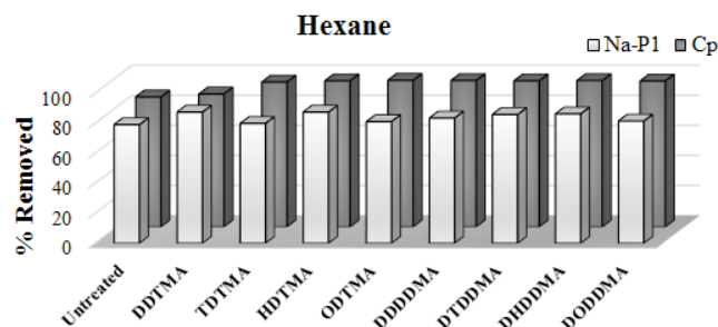
Fig. 10. Efficiency of hexane removal from aqueous solutions ( C_0 = 50 ppm, t = 2 h).
