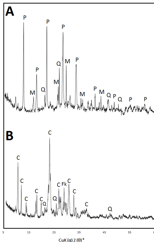
Fig. 2. X-ray diffraction patterns of: (a) – synthetic zeolite Na-P1; (b) – natural zeolite clinoptilolite.
